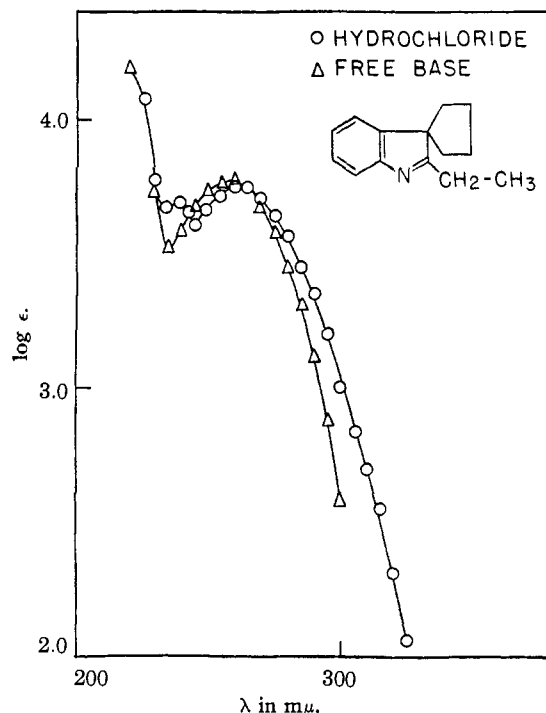
Fig. 2.—Ultraviolet spectrum of spiro -(cyclopentane-1,3'- pseud -2'-ethylindole) (free base and hydrochloride) in ethyl alcohol.
