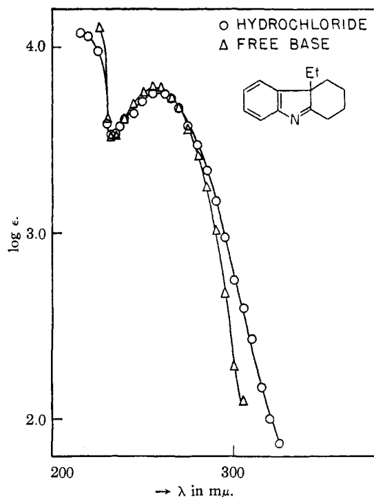
Fig. 1.—Ultraviolet spectrum of 11-ethyltetrahydrocarbazolenine (free base and hydrochloride) in ethyl alcohol.
